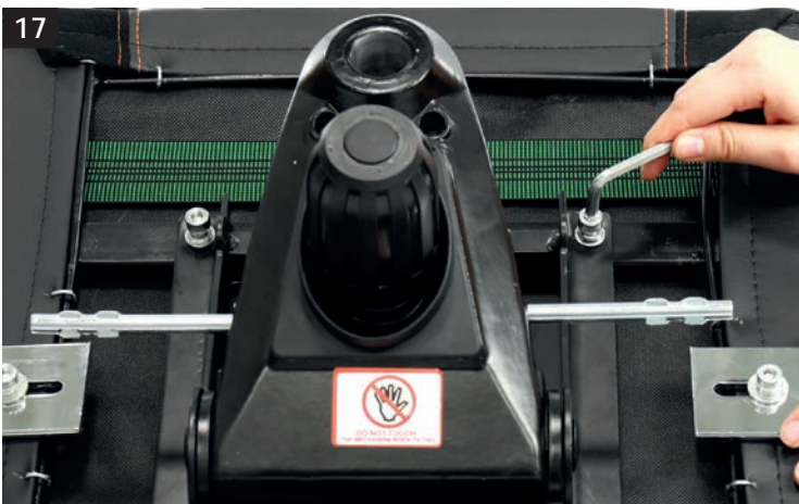
17 Then tighten the screws crosswise with the universal tool.
